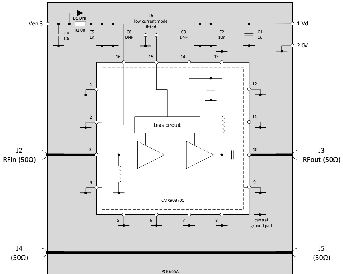
Figure 62: EV90B701 Schematic
